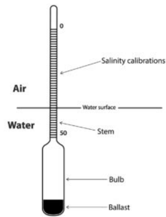
Fig. 2: A density hydrometer.
