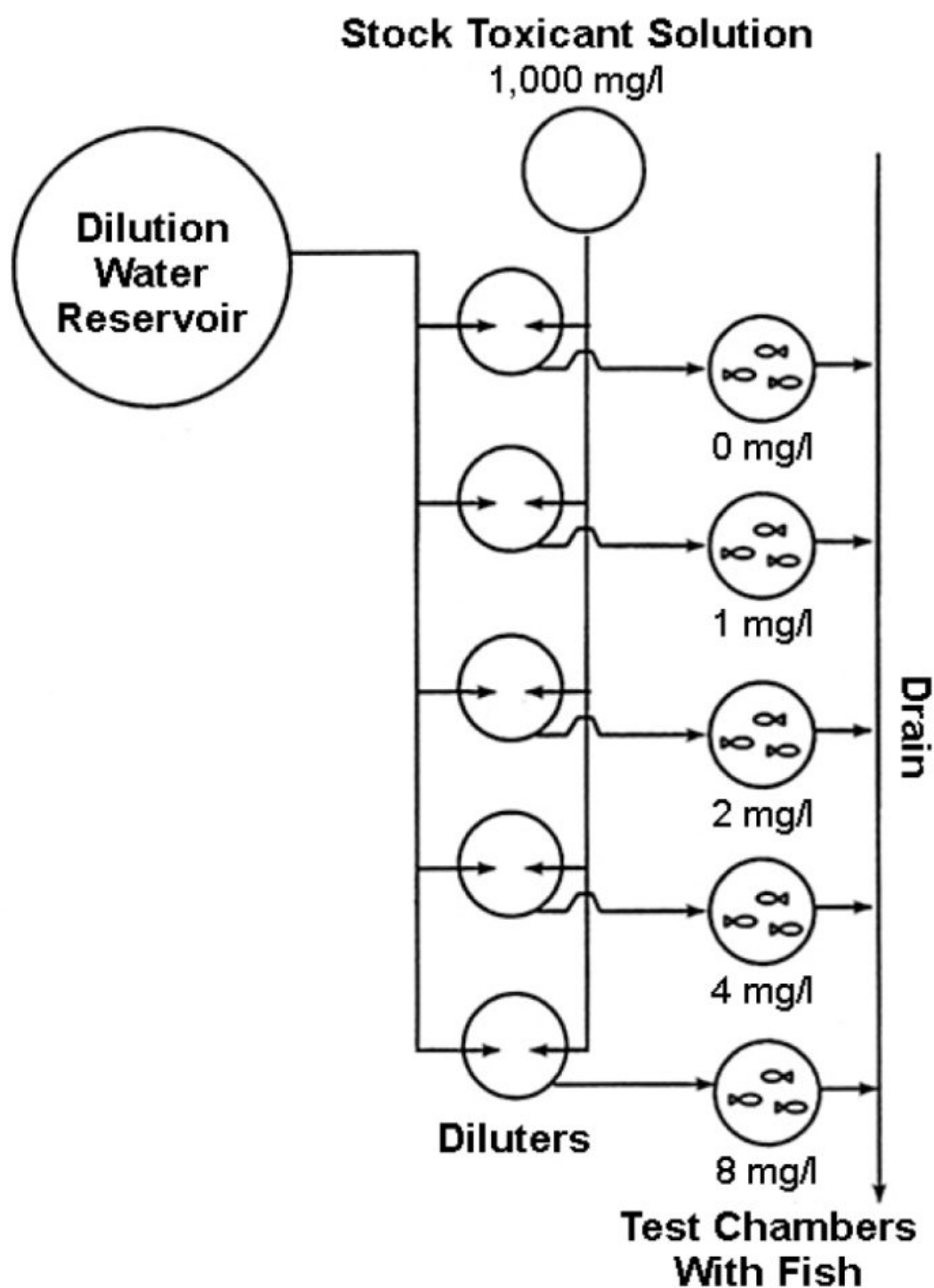
Fig. 2: Example of a flow-through toxicity test.
