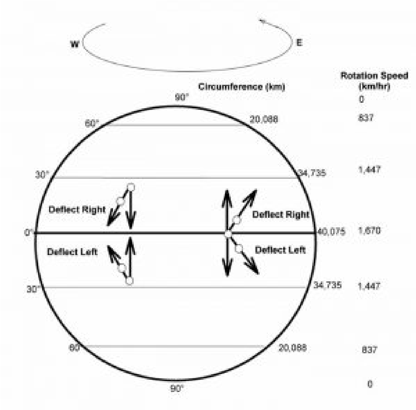
Fig. 1. Illustration of the Coriolis effect caused by the earth's rotation. The open dots represent a helicopter initially hovering motionless above the ground and then moving directly northward or southward.
