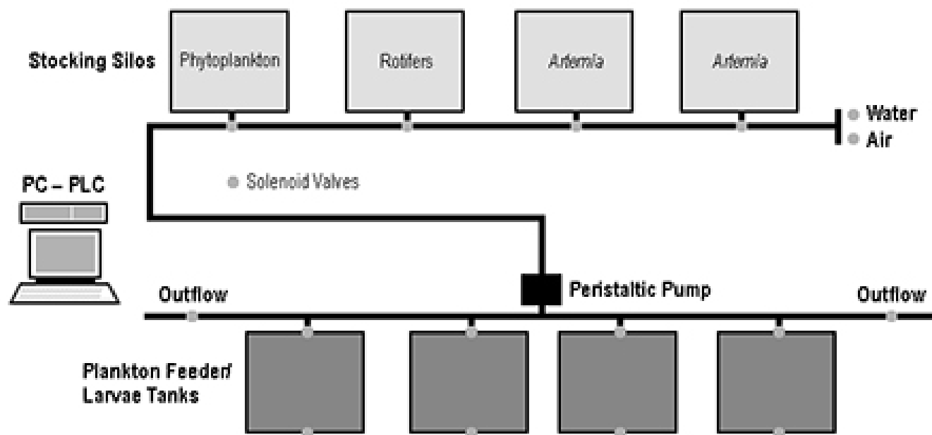
Diagram of the IMBC feeding system, with live food tanks (phytoplankton, rotifers, and Artemia) and automated feeding equipment, including the transferring circuit.
